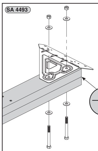
(6) \frac{3}{8} " x 3\frac{1}{2} "
